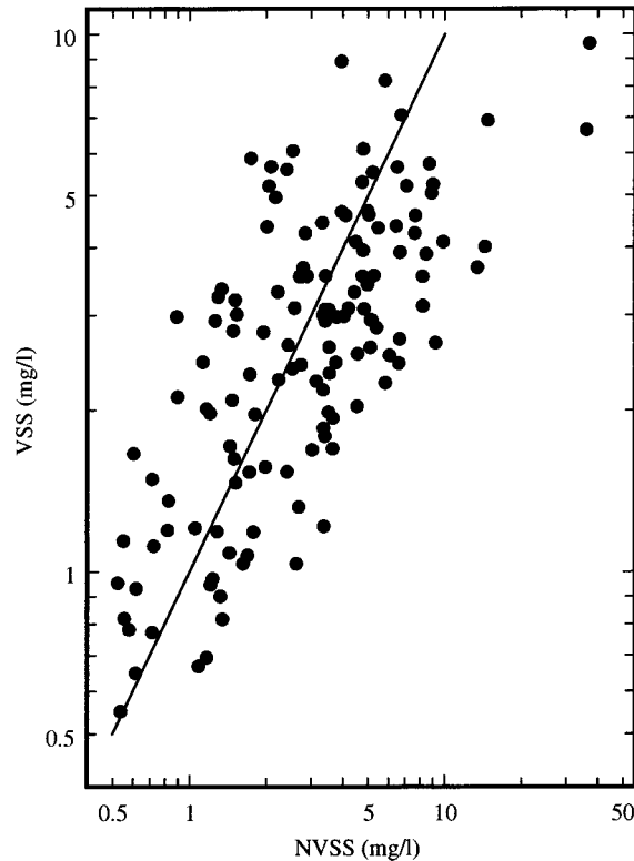
Fig. 2. Relation of mean VSS to mean NVSS from 135 Missouri reservoirs. The solid line marks a 1:1 ratio of concentrations.
