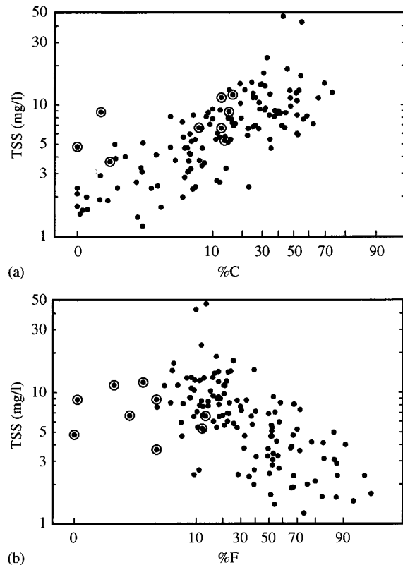
Fig. 4. Mean TSS for Missouri reservoirs versus percent cover of (a) cropland (%C, r = 0.74 ) and (b) forest (%F, r = -0.59 ) in reservoir catchments. Circled observations are for water bodies with catchments including >50% urban cover.
