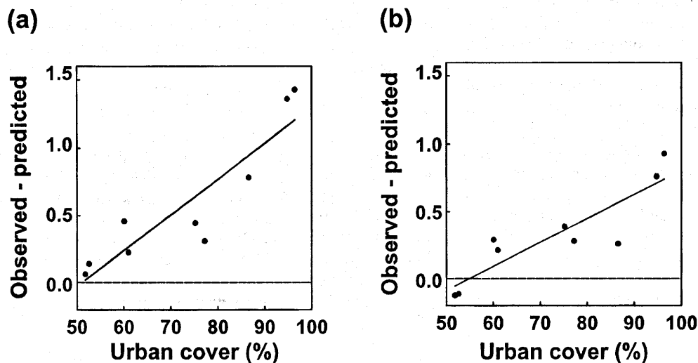
Fig. 5. Effect of the proportion of urban cover on residuals (observed – predicted, ln-transformed data) from models 3 (a; r = 0.91 ) and 5 (b; r = 0.89 ) in Table 2 calculated for nine urban reservoirs not included in the statewide land cover – nutrient analysis. Solid lines were fitted by least squares.
