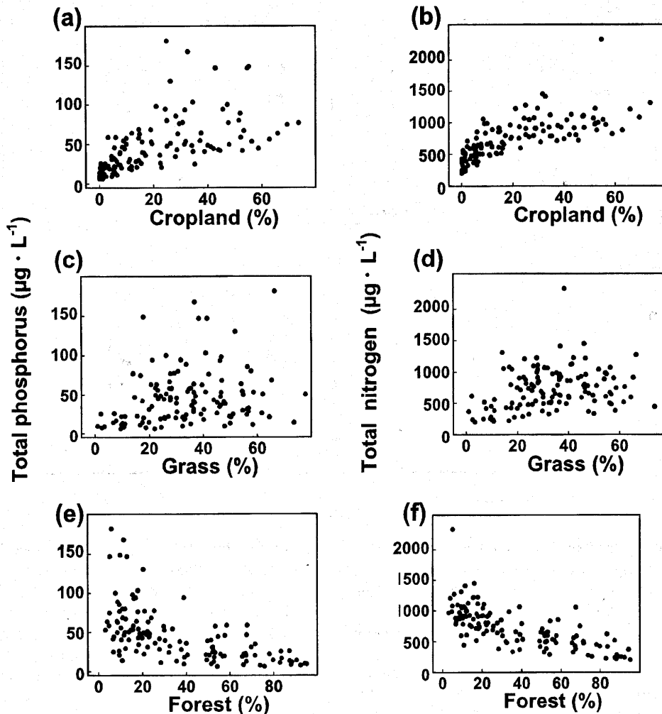
Fig. 3. Linear plots of total phosphorus and total nitrogen against the proportions of cropland, grass, and forest in the catchments.
