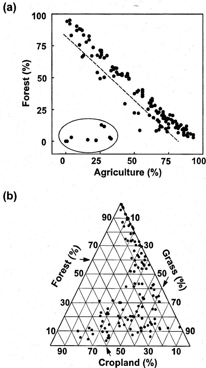
Fig. 2. (a) Plot of the proportion of forest cover in the catchments of 135 Missouri reservoirs against the proportion of the catchment in agriculture (cropland plus grass). The nine data points enclosed by an ellipse have >50% urban area in the catchment. The broken line represents 85% land cover jointly in forest and agriculture. (b) Ternary diagram showing the proportions of cropland, forest, and grass in the catchments of the Missouri reservoirs.
